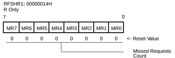
Figure 48. Refresh Register 1
