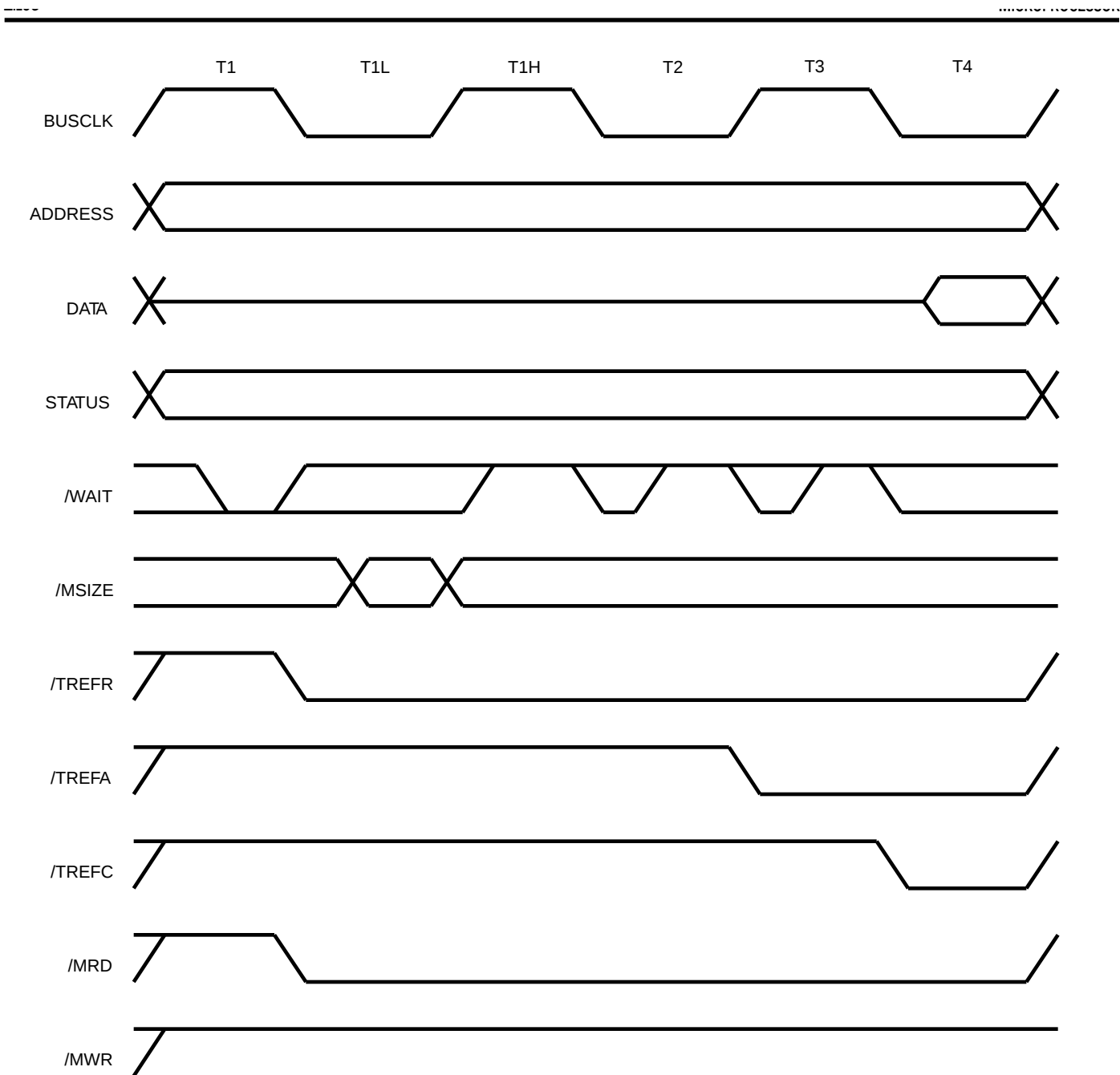
Figure 3B. Read Cycle, T1 Wait
