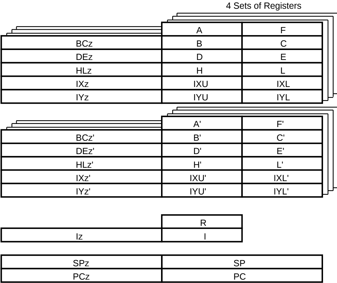
Figure 21. Register Set
