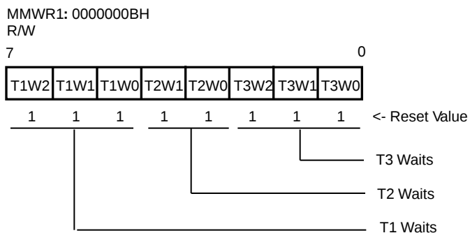
Figure 43. Mid-range Memory Waits Register 1
