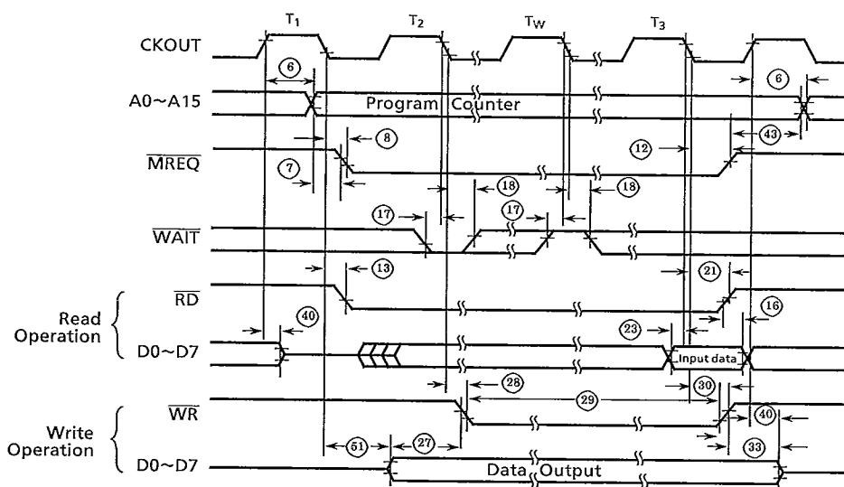
Figure 4.4.2 Memory Read/Write Cycle
