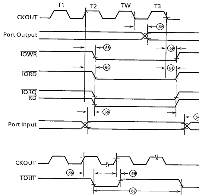
Figure 4.4.9 Input/Output Timing
