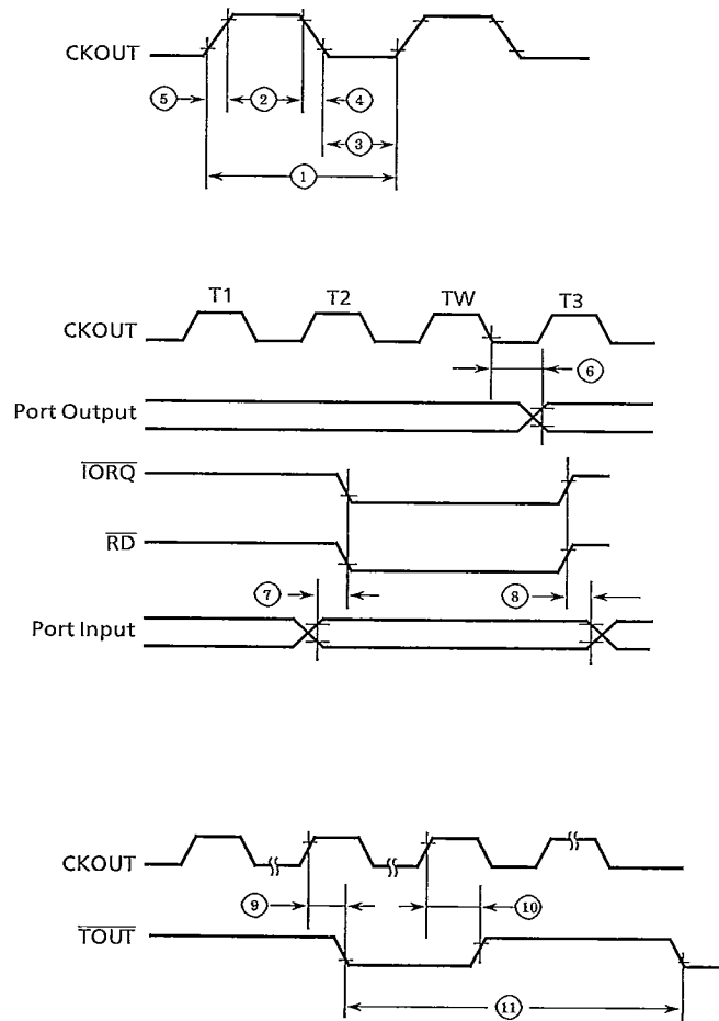
Figure 4.6.1 Input/Output Timing
