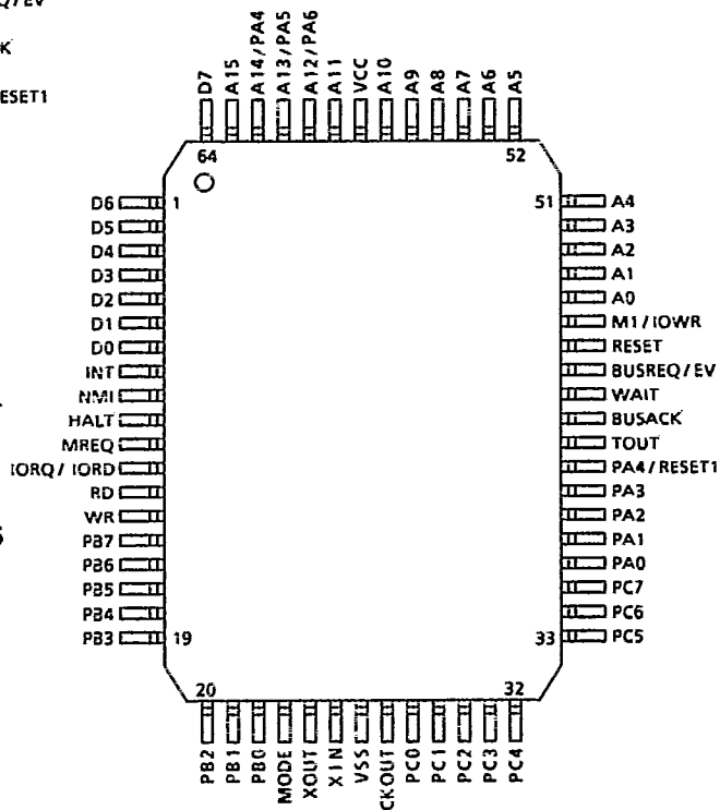
Figure 2.2 TMPZ84C112AF-6
