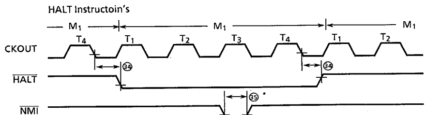
Figure 4.4.7 HALT Acknowledge Cycle
