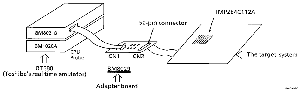
Figure 3.4.13 Typical connection
