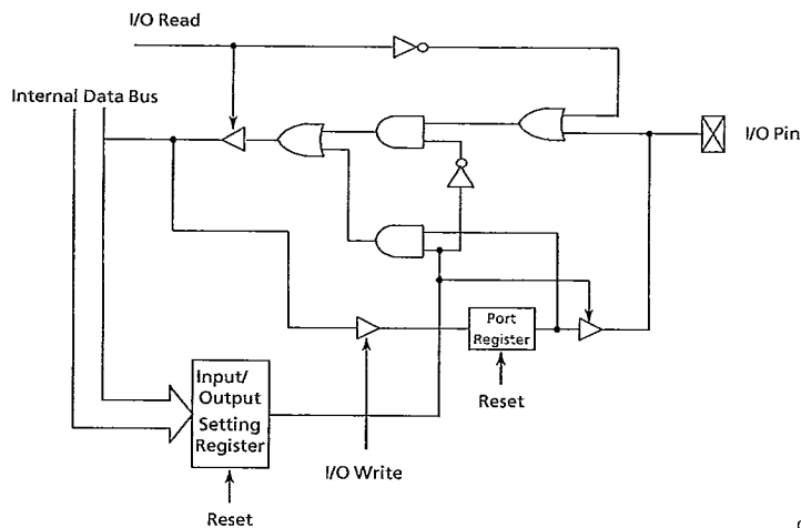
Figure 3.4.3 I/O Port Logic
