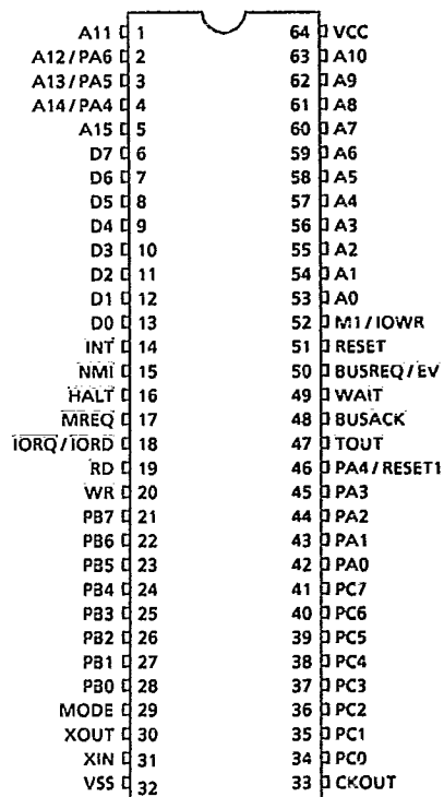
Figure 2.1 TMPZ84C112AN-6
