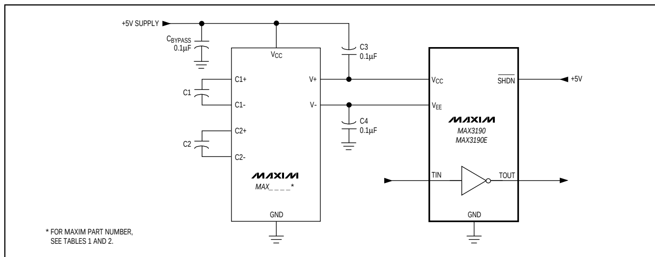
Figure 4. Powering the MAX3190/MAX3190E
