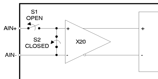
Figure 10. Self Calibration of Offset (Low Ranges).
