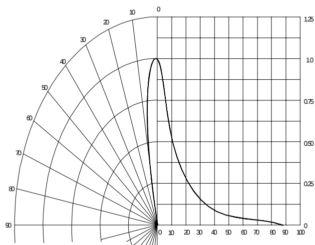
Relative Luminous Intensity vs. Angular Displacement
