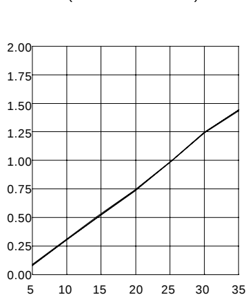
Relative Luminous Intensity vs Forward Current (Normalized at 25mA)
