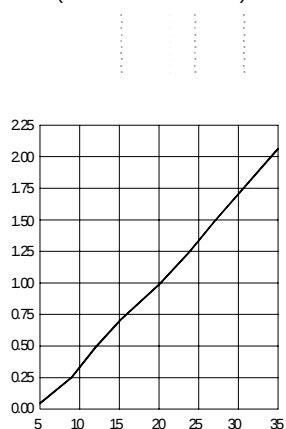
Relative Luminous Intensity vs Forward Current (Normalized at 20mA)
