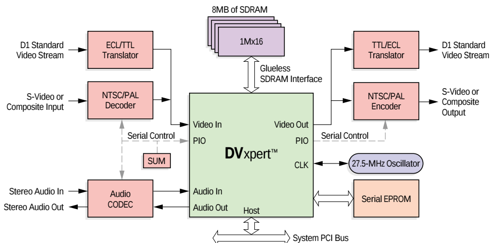
DVxpert™ 6110 Single-Chip Professional Encoder Architecture
