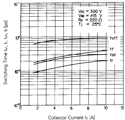
Switching Time
