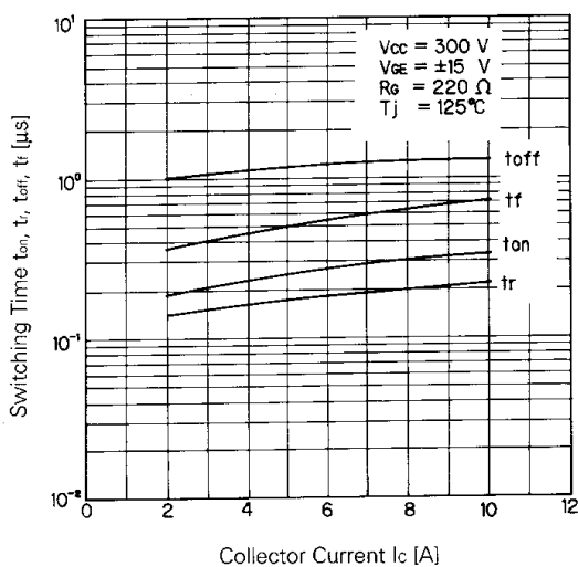
Switching Time
