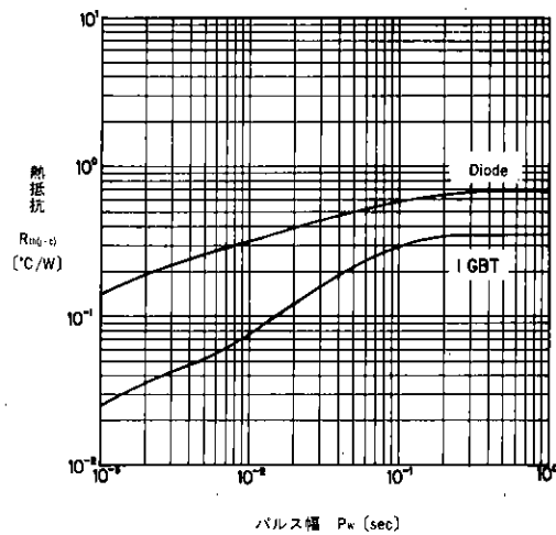
過渡熱抵抗 Transient Thermal Resistance
