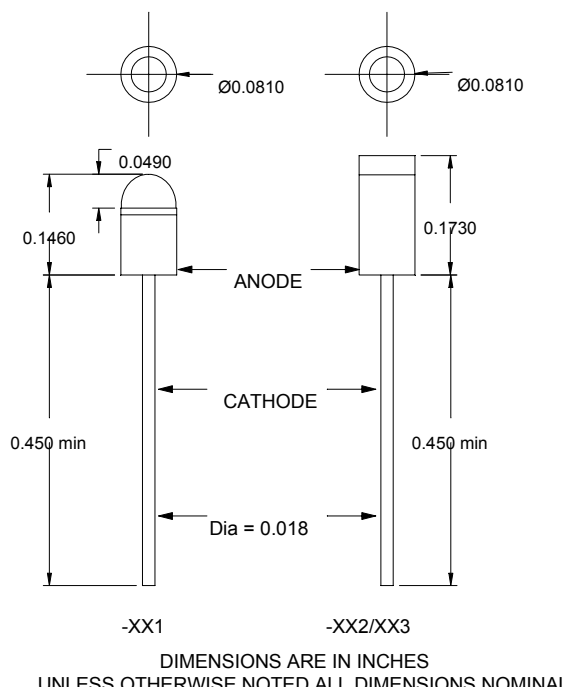
Package Dimensions
