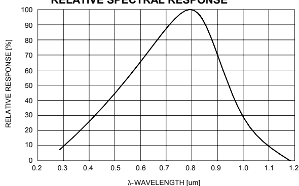
RELATIVE SPECTRAL RESPONSE
