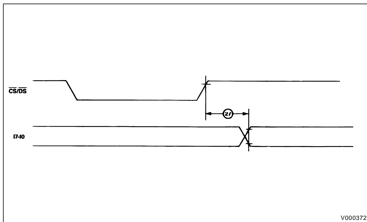
Figure 26 : Port Timing.
