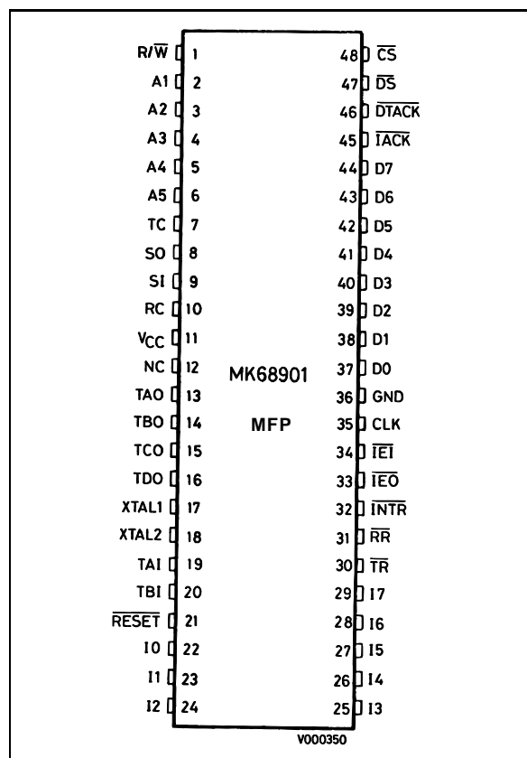
Figure 1 : Pin connections.
