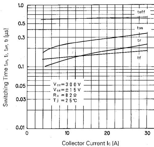
Switching Time
