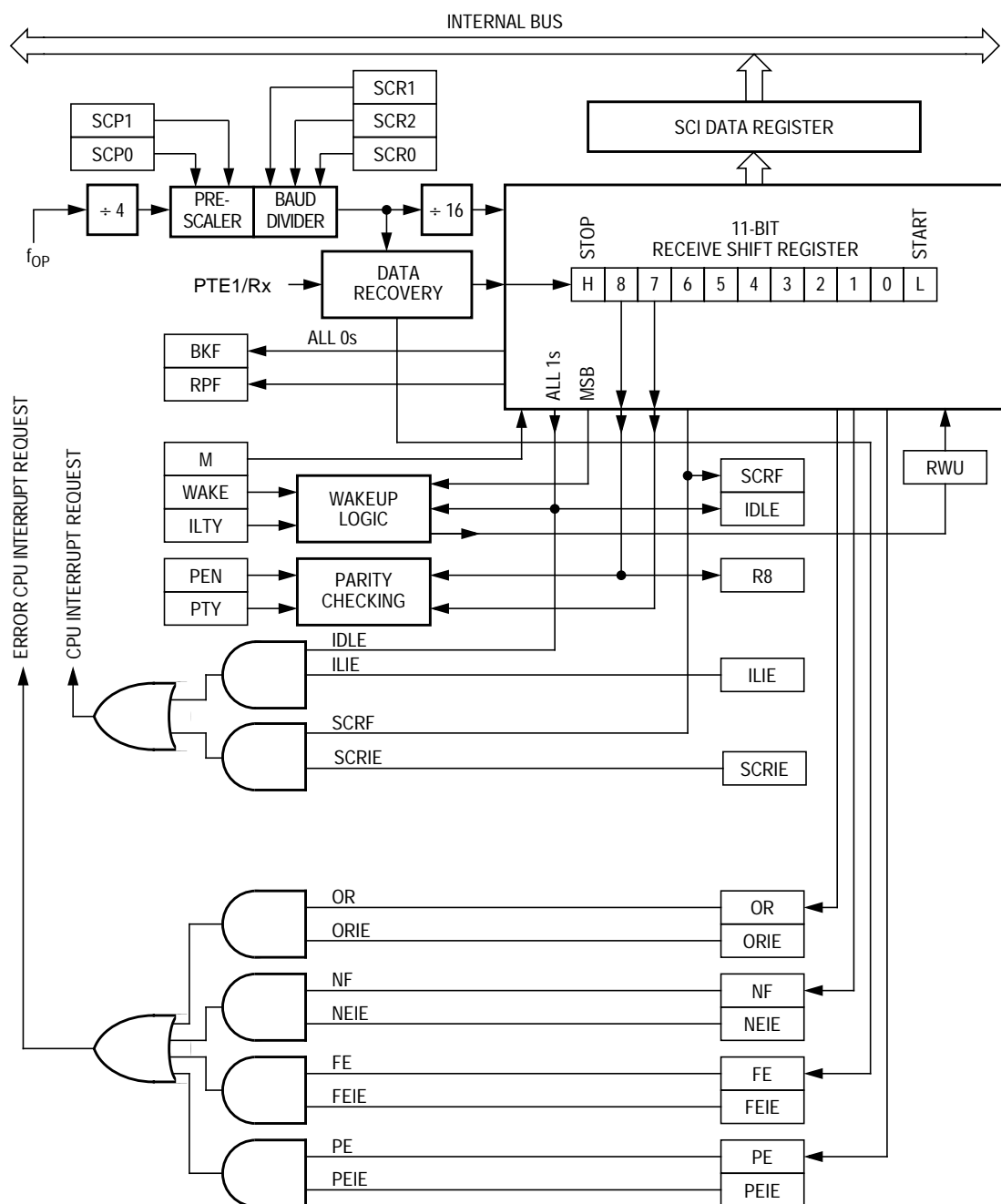
Figure 14-5. SCI Receiver Block Diagram
