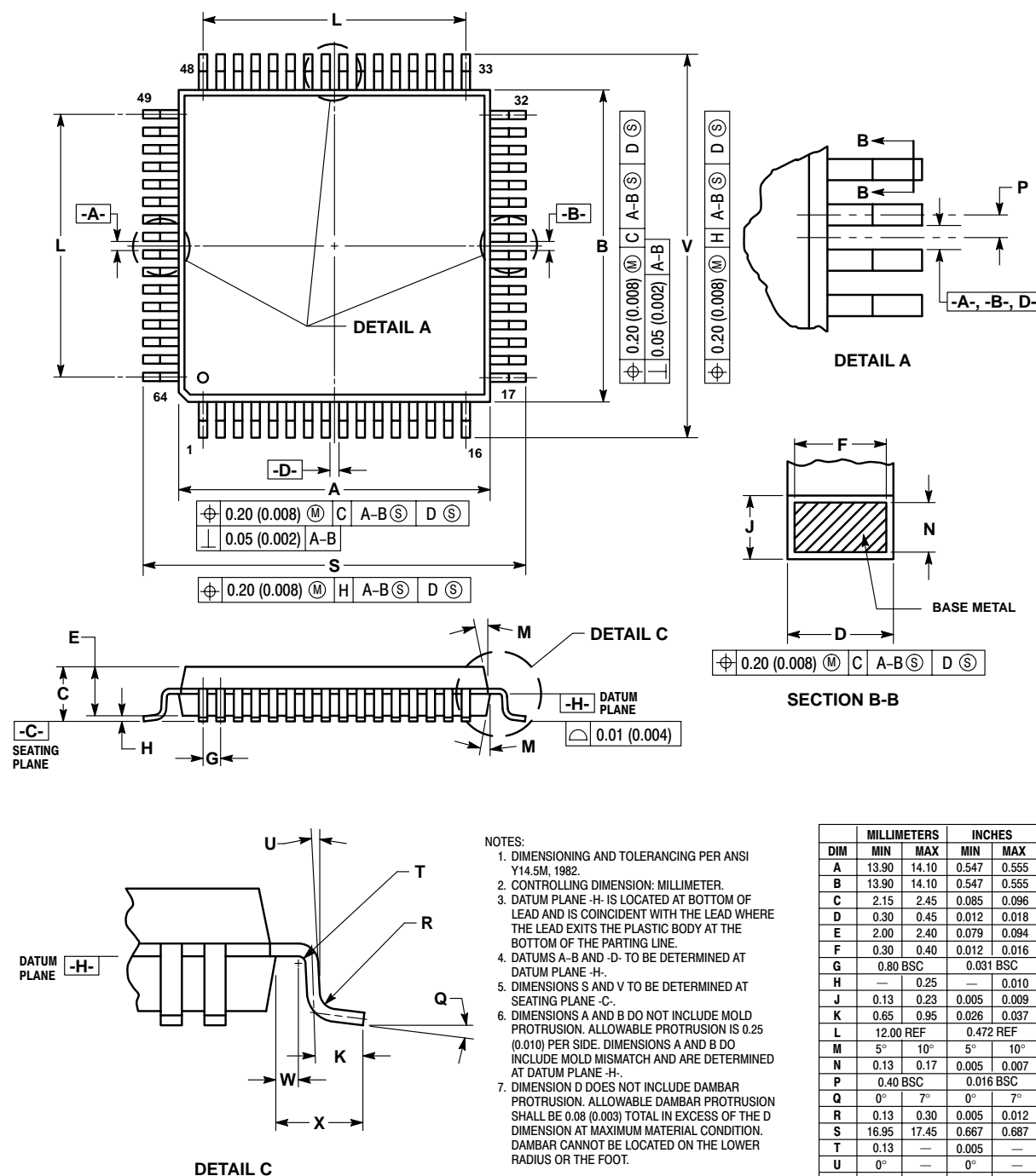
Figure 22-1. MC68HC908MR24FU
