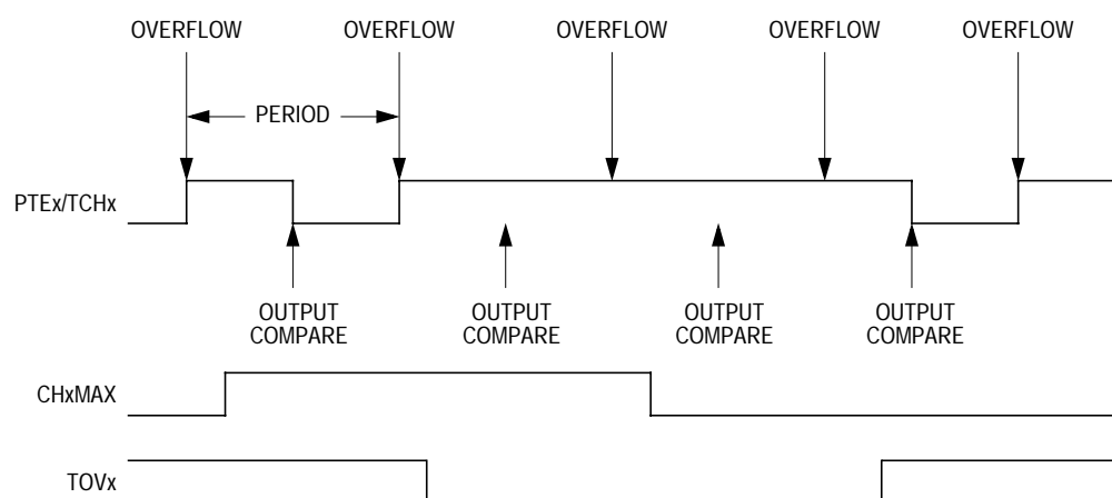
Figure 11-8. CHxMAX Latency
