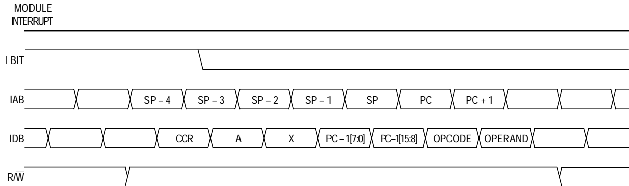
Figure 7-9. Interrupt Recovery
