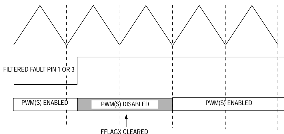
Figure 9-28. PWM Disabling in Manual Mode (Example 1)
