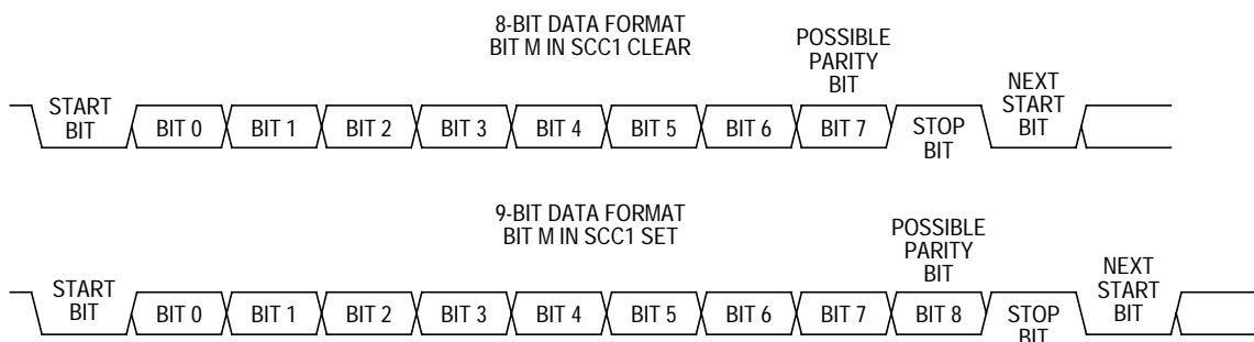
Figure 14-3. SCI Data Formats
