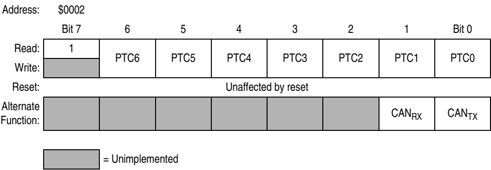
Figure 17-9. Port C Data Register (PTC)
