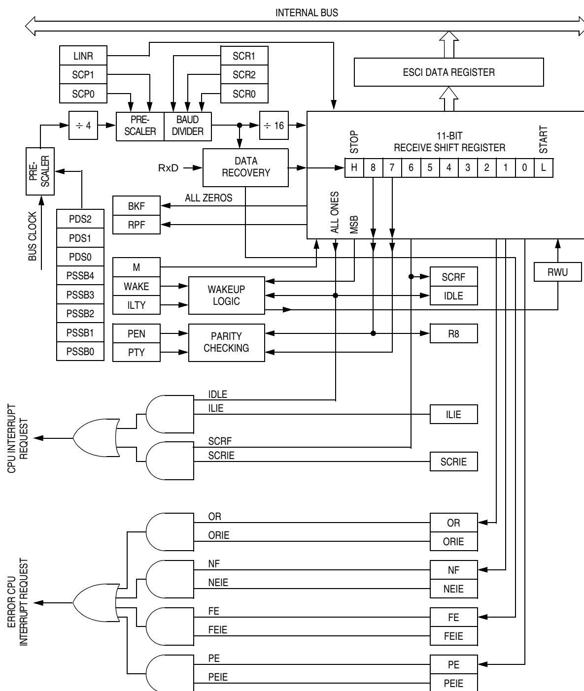
Figure 19-5. ESCI Receiver Block Diagram
