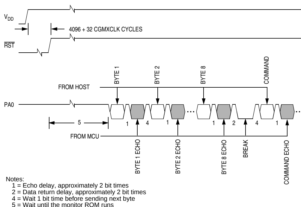
Figure 15-9. Monitor Mode Entry Timing
