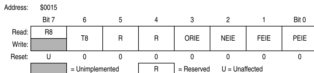
Figure 19-11. ESCI Control Register 3 (SCC3)
