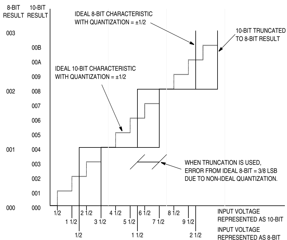
Figure 5-2. Bit Truncation Mode Error
