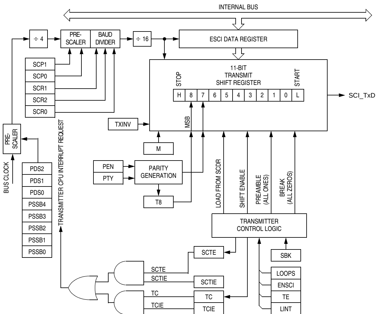
Figure 19-4. ESCI Transmitter
