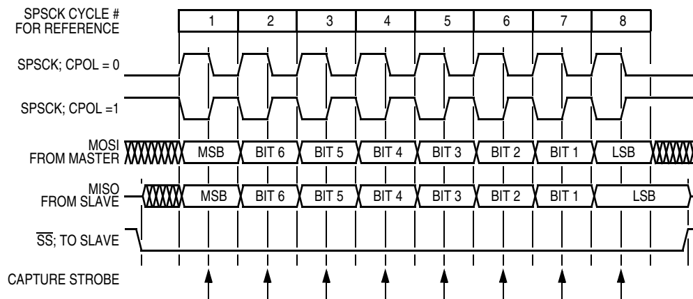
Figure 21-6. Transmission Format ( \text{CPHA} = 1 )
