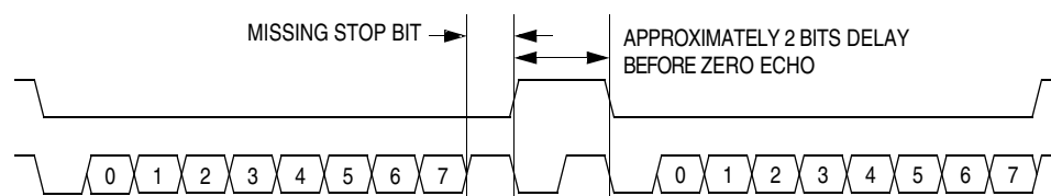
Figure 15-5. Break Transaction
