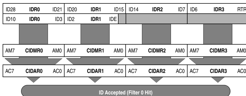
Figure 16-3. Single 32-Bit Maskable Identifier Acceptance Filter
