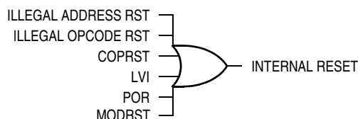
Figure 20-6. Sources of Internal Reset
