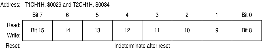
Figure 23-14. TIM Channel 1 Register High (TCH1H)
