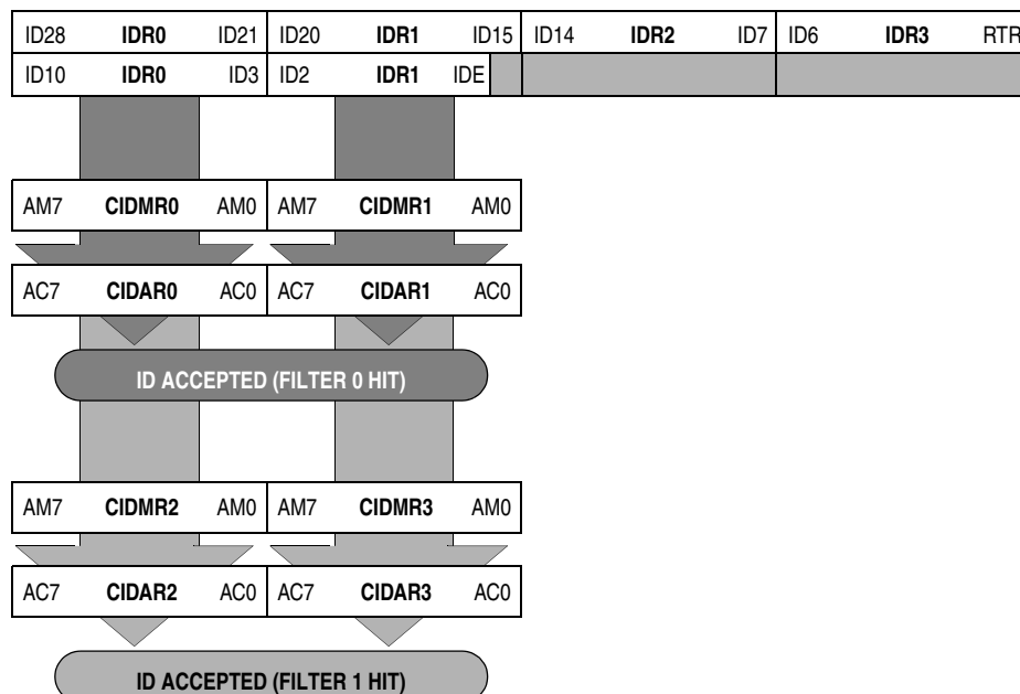
Figure 16-4. Dual 16-Bit Maskable Acceptance Filters
