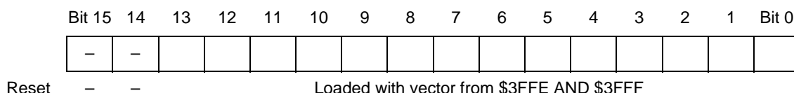
Figure 3-5 Program Counter
