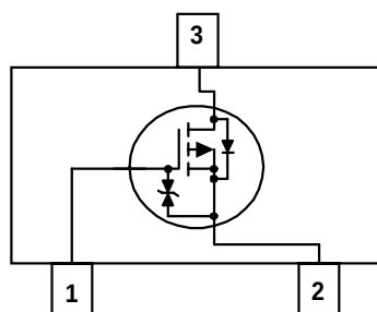
P - Channel MOS FET ( 1 device built-in )
