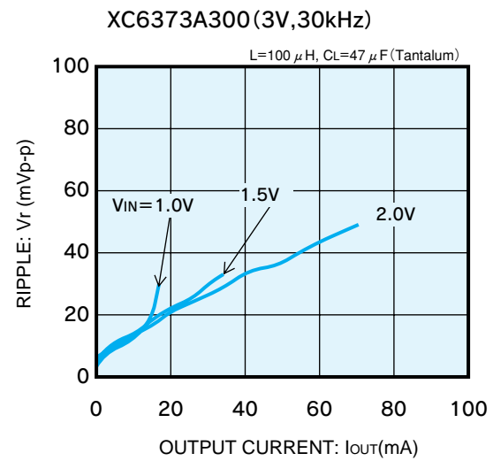
(4) RIPPLE VOLTAGE vs. OUTPUT CURRENT
