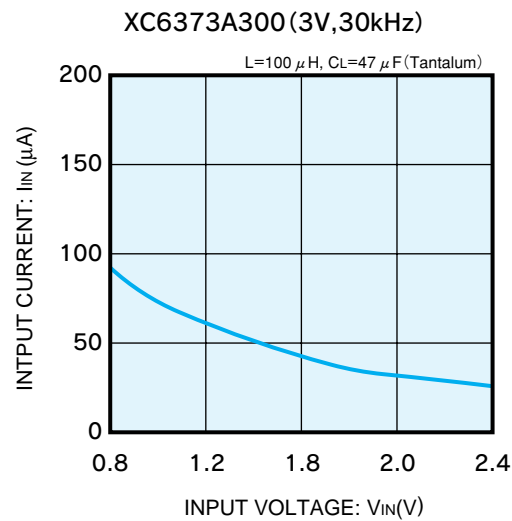
(3) NO LOAD INPUT CURRENT vs. INPUT VOLTAGE
