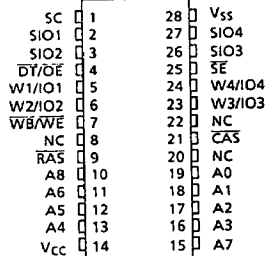
TC524256BJ
