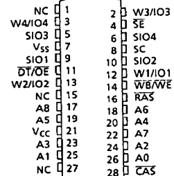
TC524256BZ
