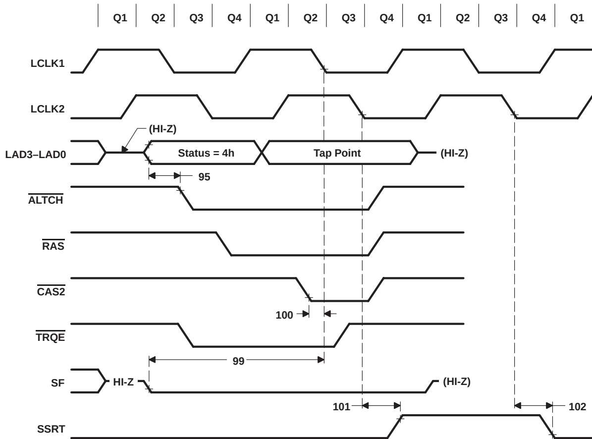
Figure 14. Shift Register Transfer Decode
