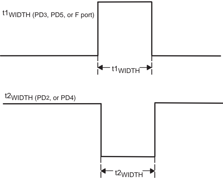
Figure 2. MSP50P604 External Interrupt Pin Pulse Width Requirements t1 WIDTH and t2 WIDTH
