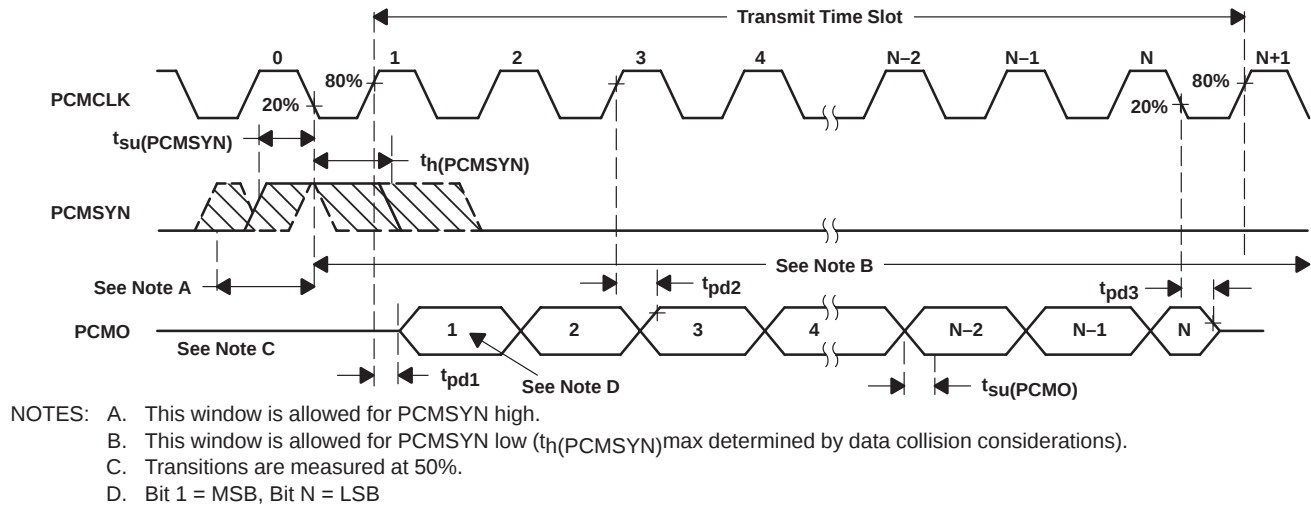
Figure 5. Transmit Timing Diagram
