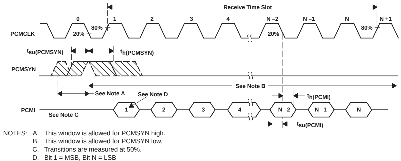
Figure 6. Receive Timing Diagram
