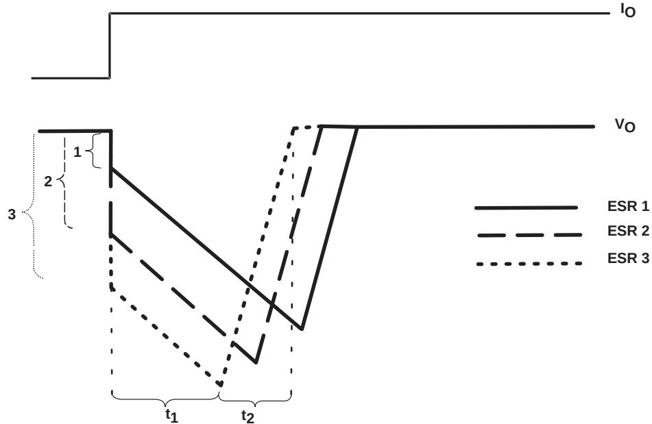
Figure 39. Correlation of Different ESRs and Their Influence to the Regulation of V_O at a Load Step From Low-to-High Output Current
