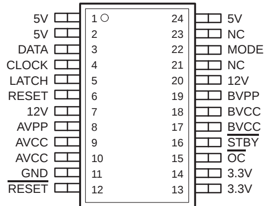
DB PACKAGE (TOP VIEW)
