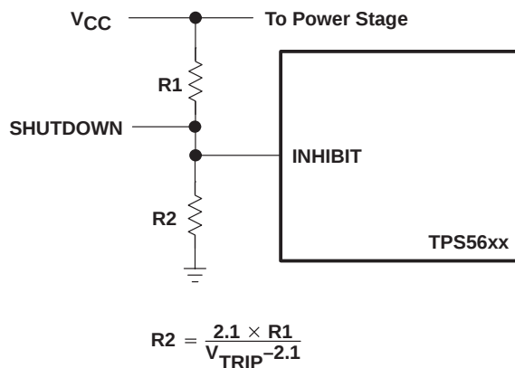
Figure 4. Input Undervoltage Lockout Circuit Using INHIBIT
