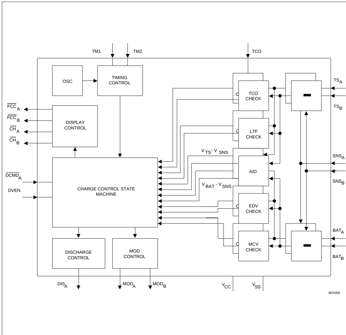
Figure 3. Block Diagram
