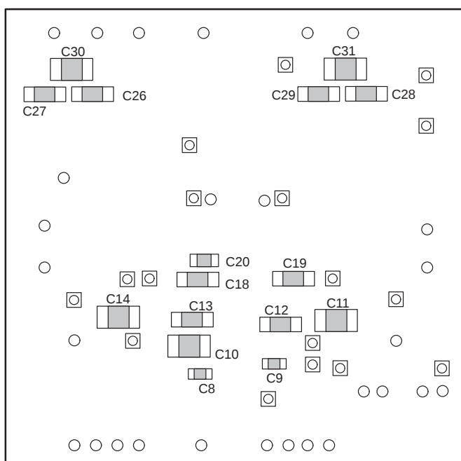
Figure 1–2. The TI TPA005D14 Class-D Stereo Audio Power Amplifier EVM — Bottom View
