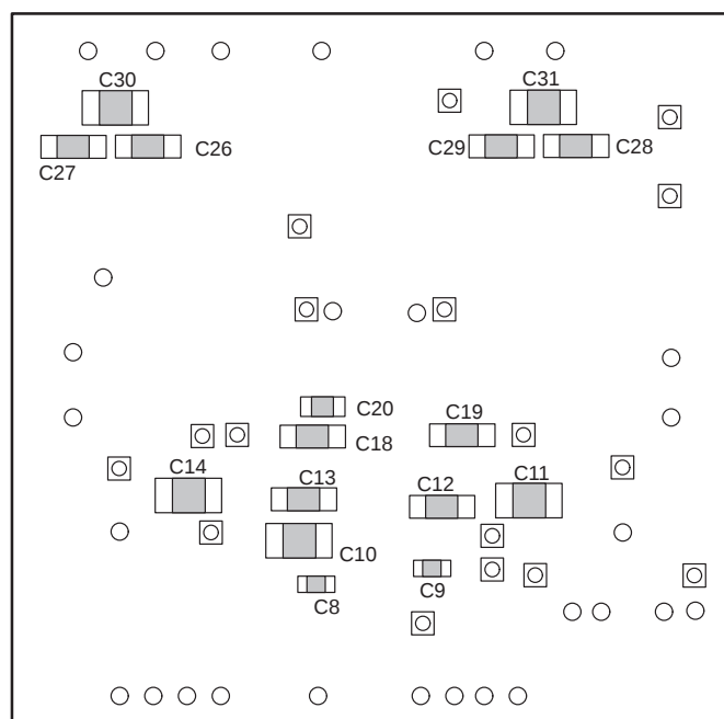
Figure 3–3. The TI TPA005D14 Class-D Stereo Audio Power Amplifier EVM — Bottom View
