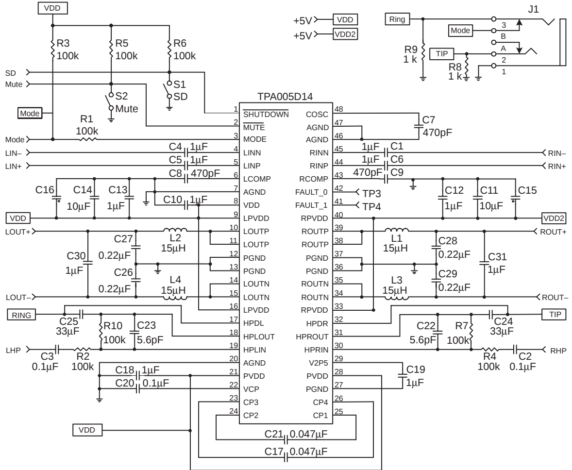
Figure 3–22. TPA005D14 Class-D EVM Schematic Diagram
