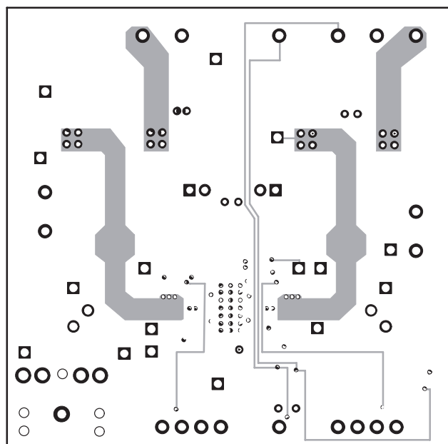
Figure 3–26. TPA005D14 Class-D EVM Second Layer
