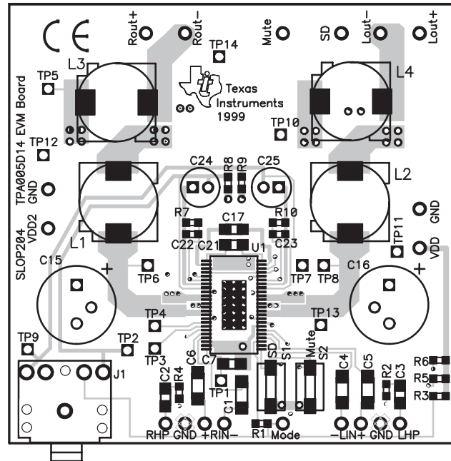
Figure 3–23. TPA005D14 Class-D EVM Top Assembly
