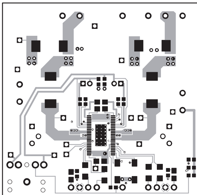
Figure 3–25. TPA005D14 Class-D EVM Top Layer
