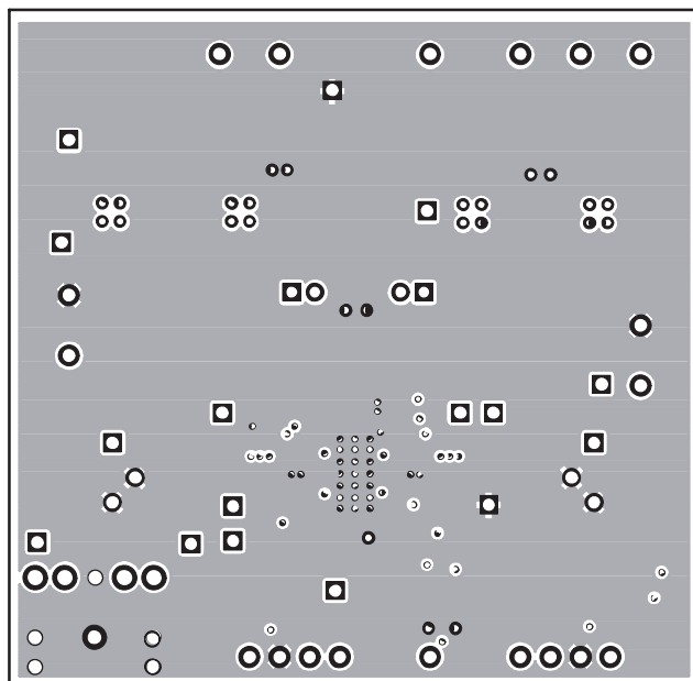
Figure 3–27. TPA005D14 Class-D EVM Third Layer
