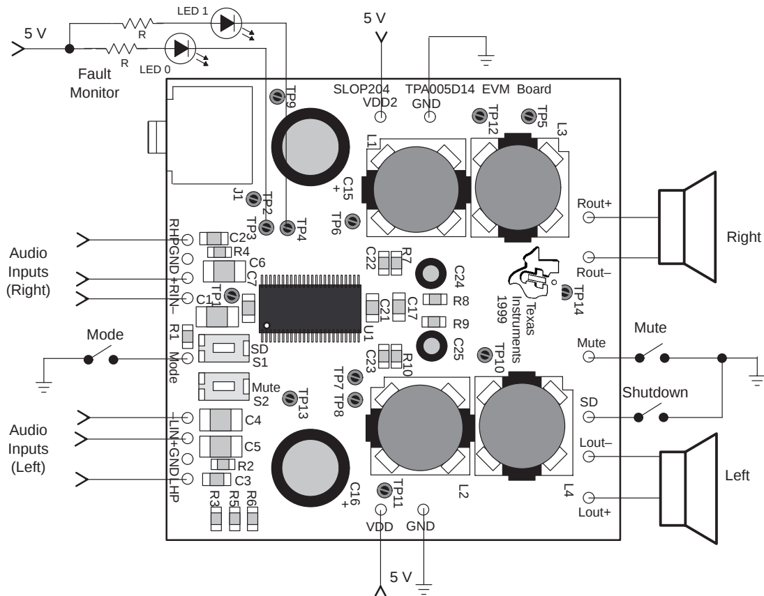
Figure 3–10. TPA005D14 Class-D EVM Stand-Alone Connections for Stereo BTL Output
