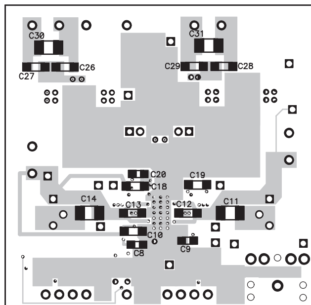
Figure 3–24. TPA005D14 Class-D EVM Bottom Assembly
