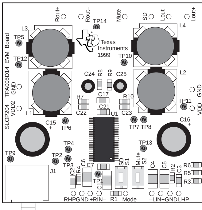
Figure 1–1. The TI TPA005D14 Class-D Stereo Audio Power Amplifier EVM — Top View
