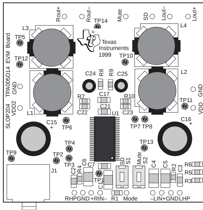
Figure 3–2. The TI TPA005D14 Class-D Stereo Audio Power Amplifier EVM — Top View
