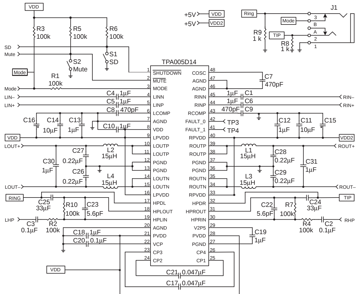
Figure 3–4. TPA005D14 Class-D EVM Schematic Diagram
