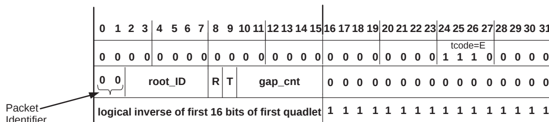
Figure 4–21. PHY-Configuration Packet Format
