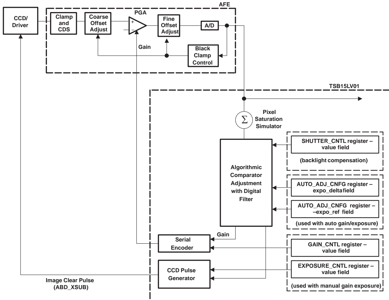
Figure 2–16. Gain and Exposure Automatic and Manual Controls
