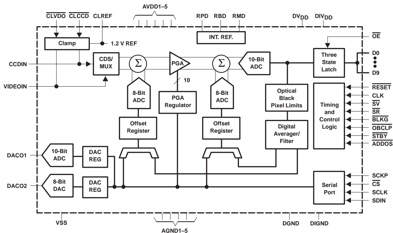
Figure 2-2. TLV990 Block Diagram
