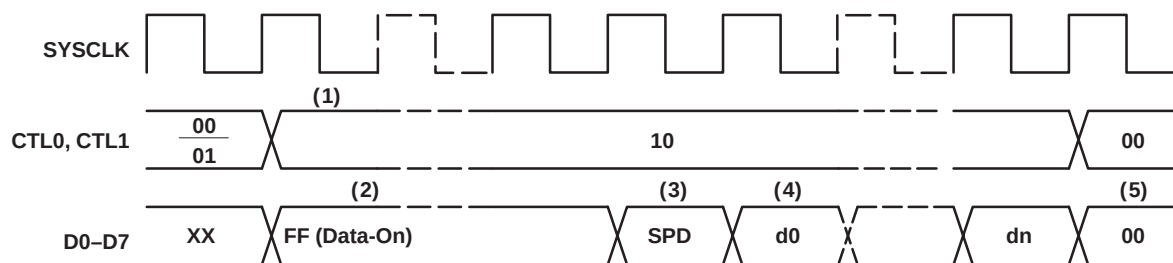
Figure 19. Normal Packet Reception Timing
