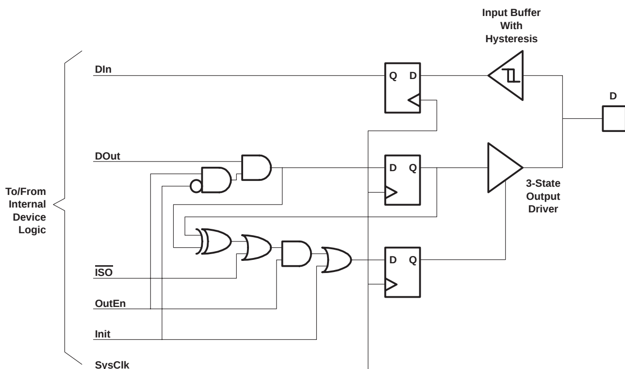
Figure 15. Signal Transformation for Digital Differentiation
