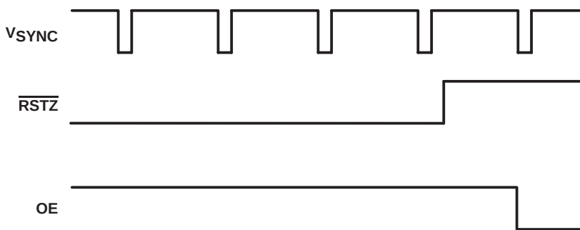
Figure 3. Reset Waveform
