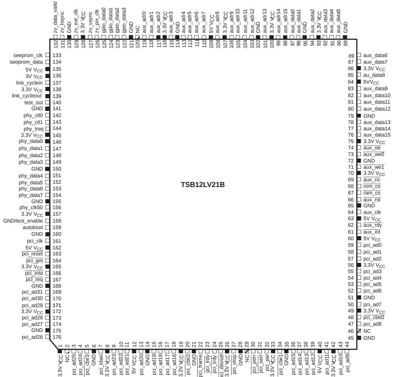
Figure 1. PCILynx-2 Terminal Assignment/Pinout
