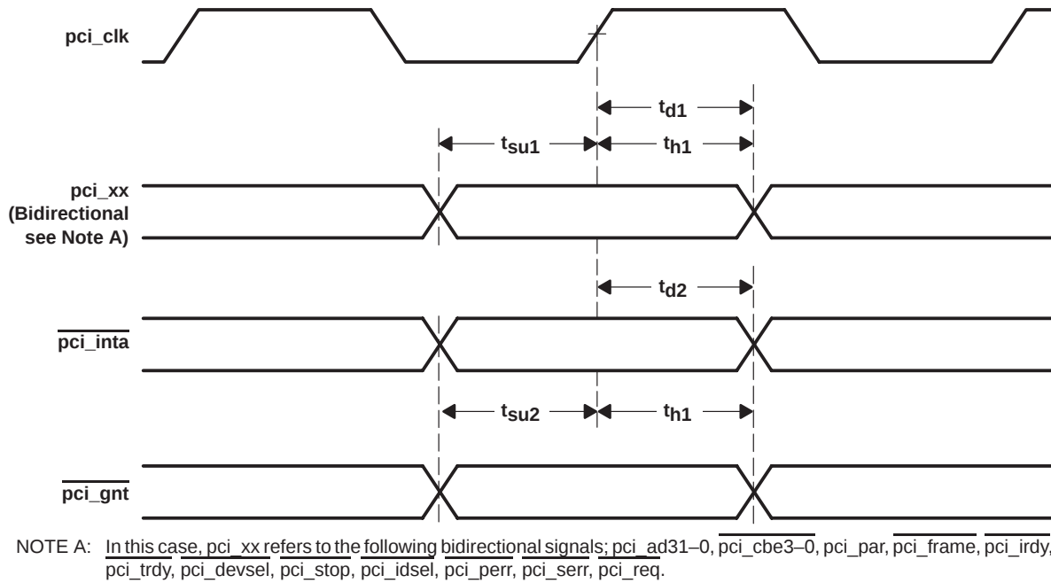
Figure 4. PCI Interface Timing Waveforms
