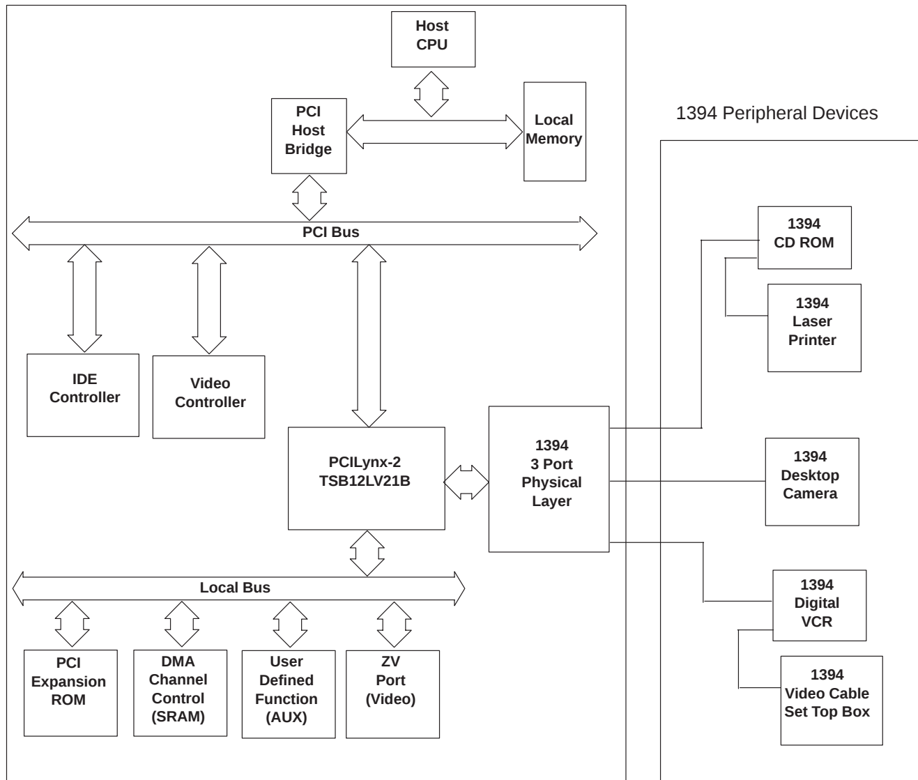
Figure 2. System Block Diagram
