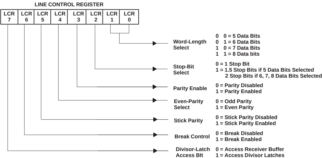
Figure 18. Line-Control Register Contents
