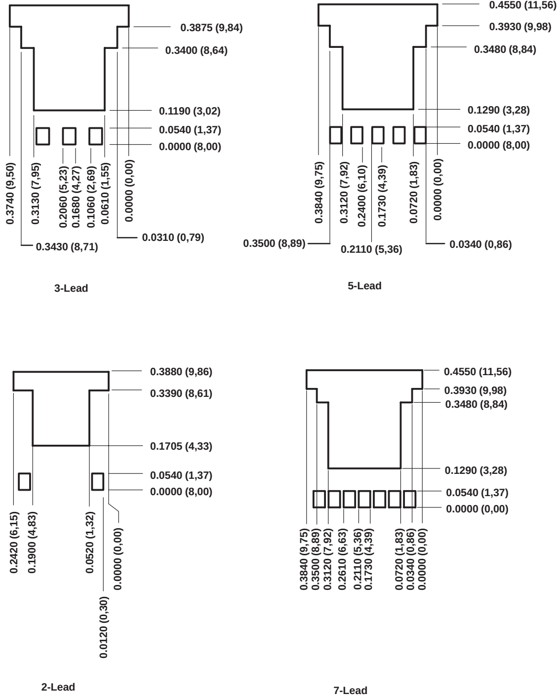
Figure 22. PowerFLEX Package Footprints
