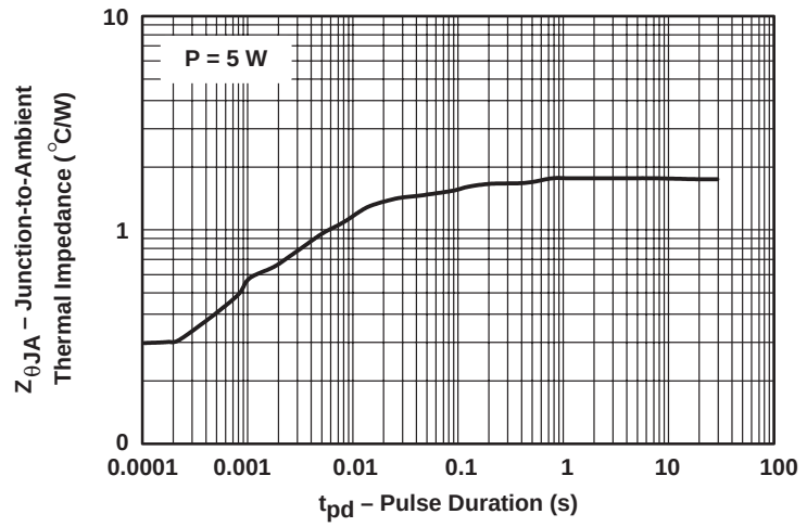
Figure 9. Transient Thermal Impedance of Device 4 in a 7-Pin PowerFLEX Package
