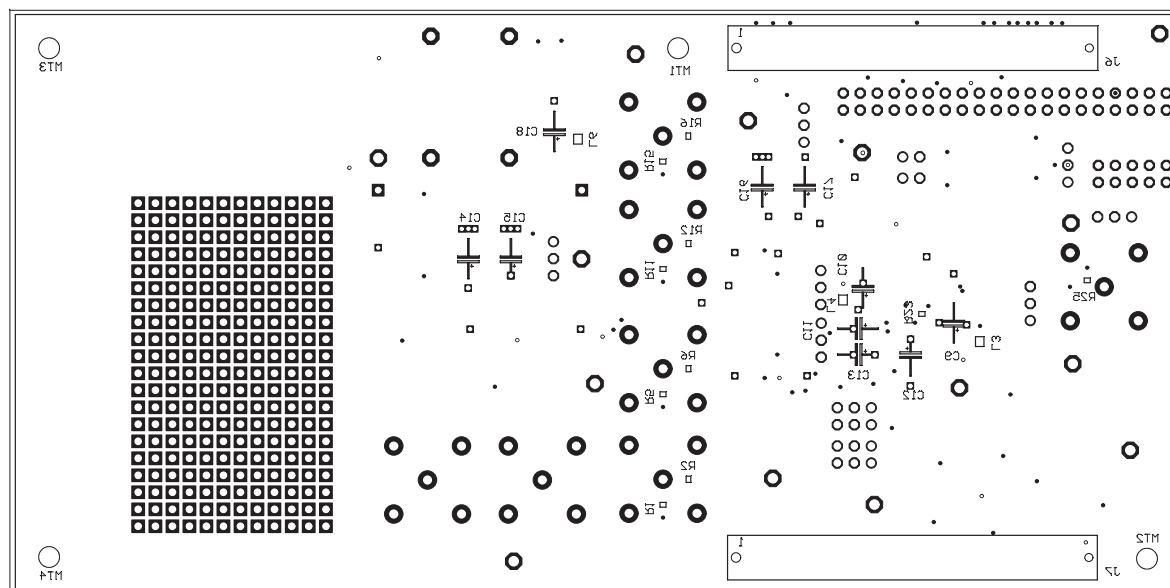
Figure 3–2. Silkscreen (Bottom)
