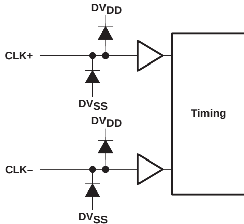
Figure 4. Clock Inputs
