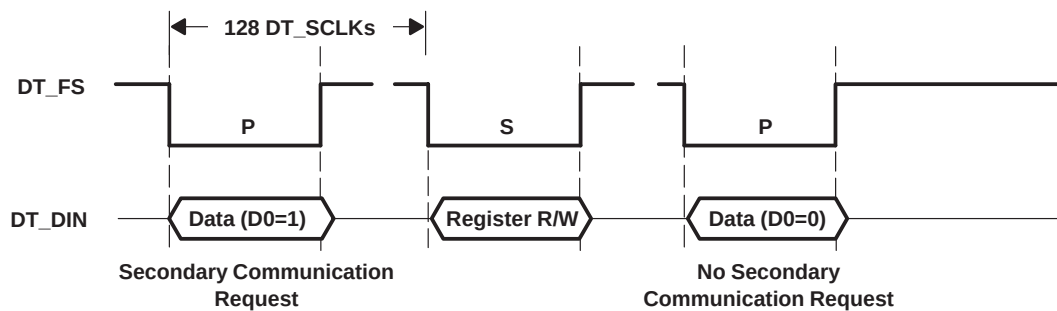
Figure 4–6. FS Output During Software Secondary Serial Communication Request (FS Low Mode)
