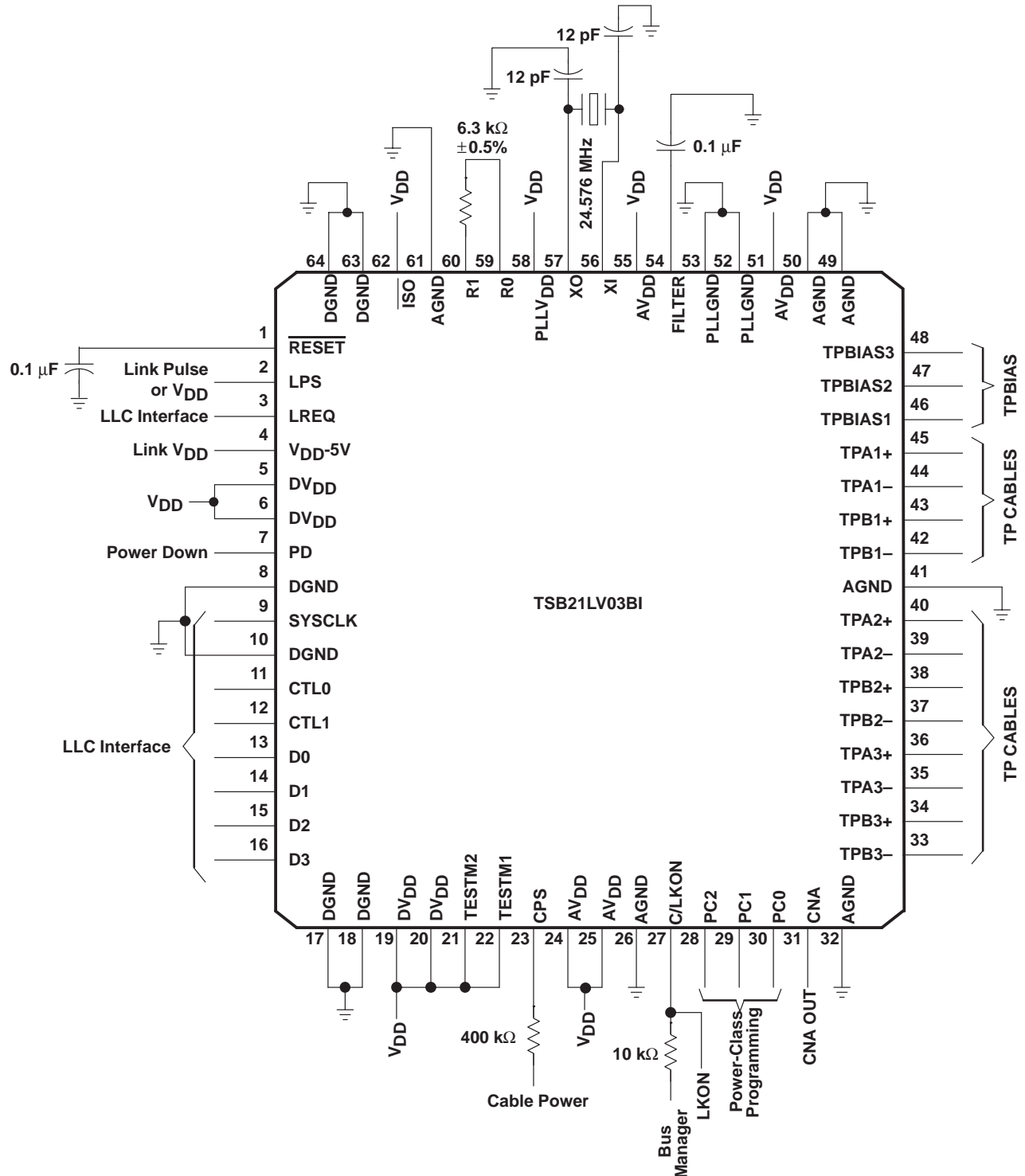
Figure 5. External Component Connections
