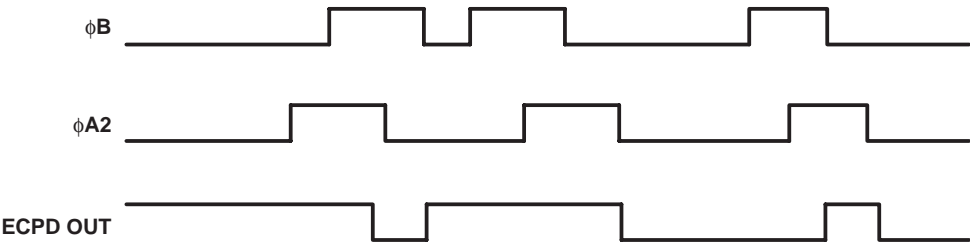
Figure 5. Edge-Controlled Phase-Comparator Waveforms
