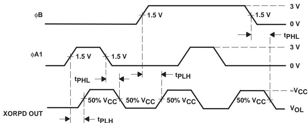
Figure 8. Waveforms Showing Phase Input ( \phi_B , \phi_{A2} ) to Output (XORPD OUT) Propagation Delays
