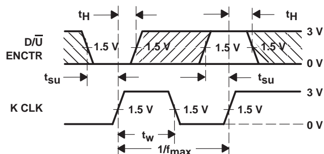
Figure 10. Waveforms Showing Clock (K CLK) Pulse Duration and Maximum Clock Pulse Frequency, and Inputs (D/U, ENCTR) to Clock (K CLK) Setup and Hold Times.
