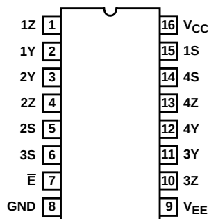
CD54HC4316 (CERDIP) CD74HC4316, CD74HCT4316 (PDIP, SOIC) TOP VIEW
