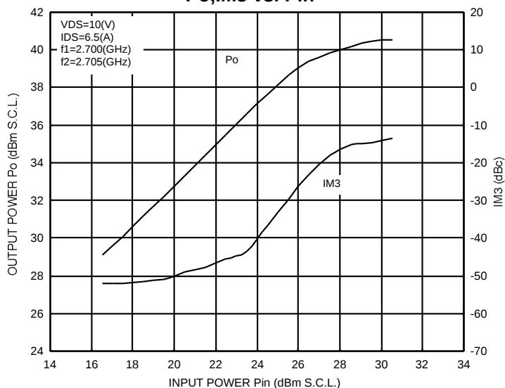
Po, IM3 vs. Pin
