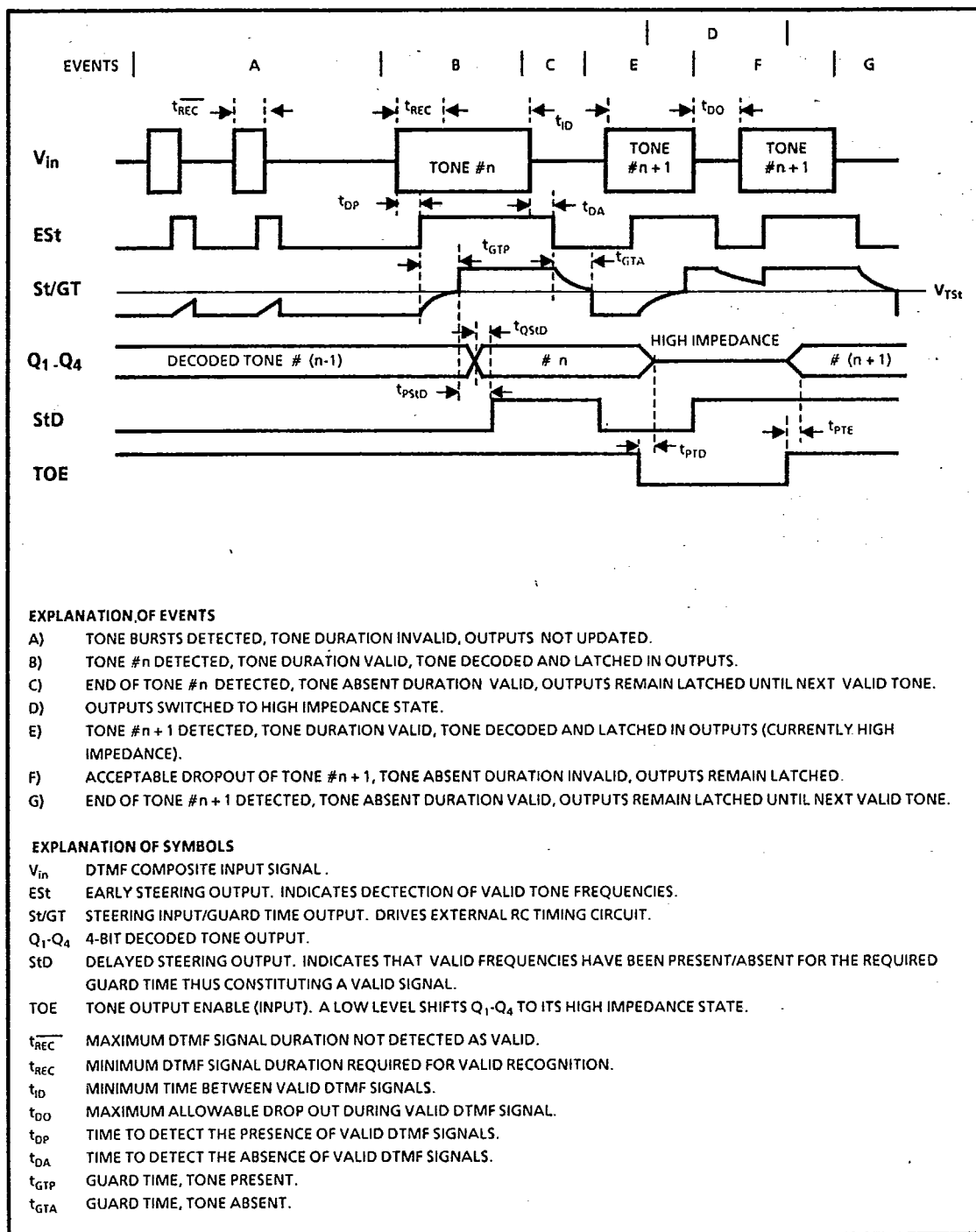
Figure 3- Timing Diagram
