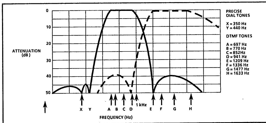
Figure 4- Filter Response
