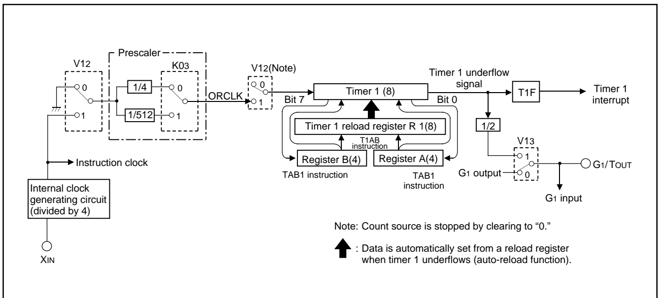
Fig. 19 Timers structure
