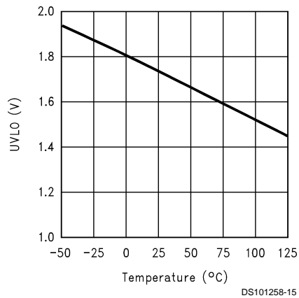
Under-Voltage Lockout (UVLO) Threshold vs Junction Temperature
