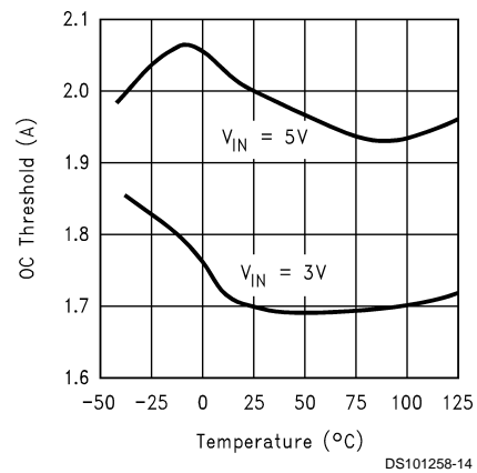
Over-Current Threshold vs Junction Temperature (Note 10)
