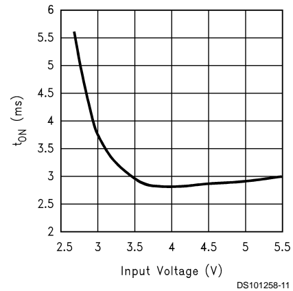
Turn-On Delay vs Input Voltage ( C_{IN} = 33\text{ }\mu\text{F} , C_{OUT} = 33\text{ }\mu\text{F} )
