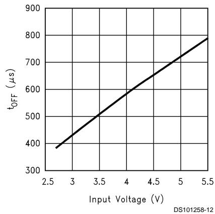
Turn-Off Delay vs Input Voltage ( C_{IN} = 33\text{ }\mu\text{F} , C_{OUT} = 33\text{ }\mu\text{F} )
