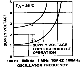
SUPPLY VOLTAGE RANGE FOR CORRECT OPERATION OF \div 8 COUNTER AS A FUNCTION OF OSCILLATOR FREQUENCY.
