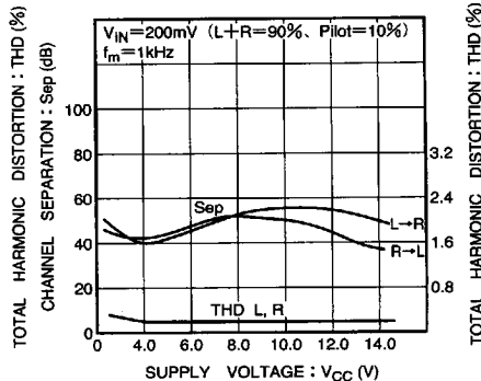
Fig. 4 Total harmonic distortion and channel separation vs. supply voltage
