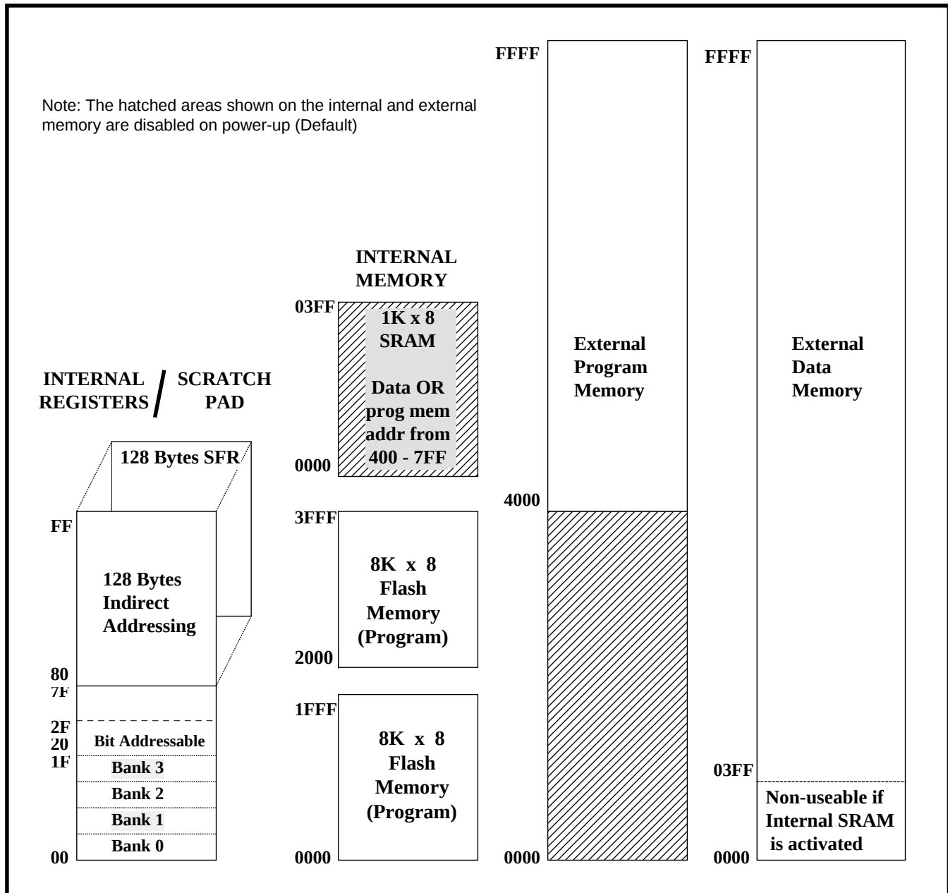
MEMORY MAP Figure 2
