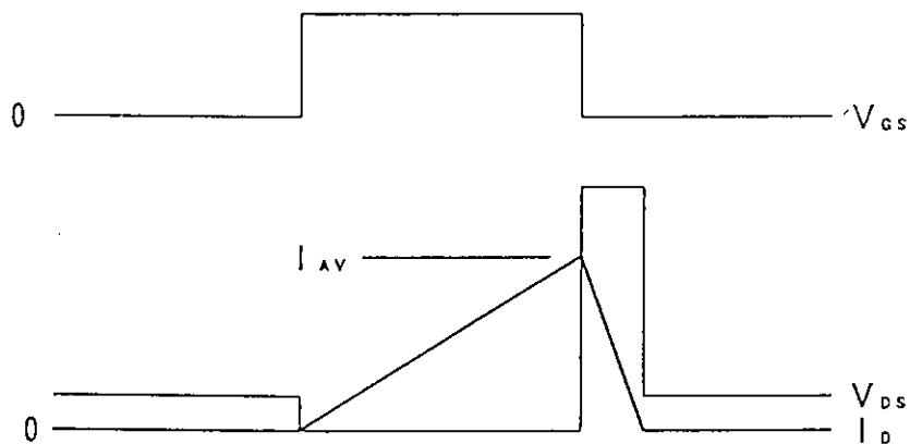
Fig.2 Operating waveforms
