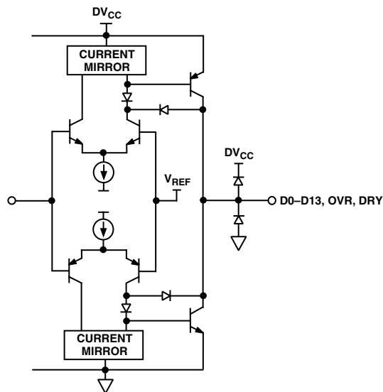
Figure 5. Digital Output Stage
