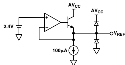
Figure 6. 2.4 V Reference
