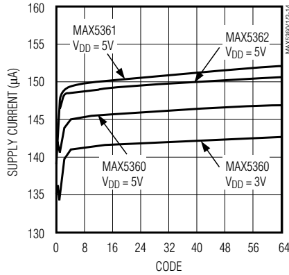
SUPPLY CURRENT vs. CODE
